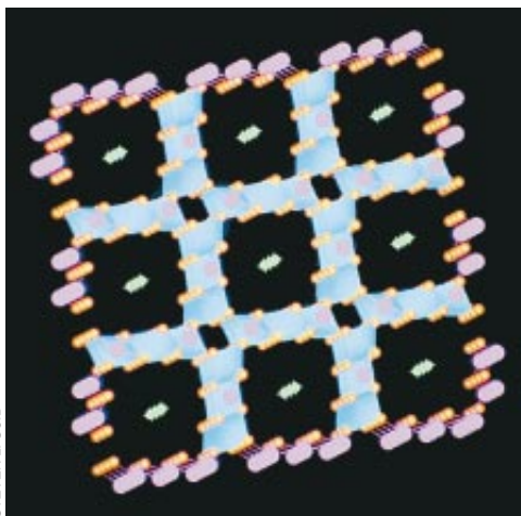
TUNNELS of synthetic todorokite, made of manganese (pink) and oxygen (orange) atoms, have each adsorbed a calcium ion (green) in this computer-generated image.
